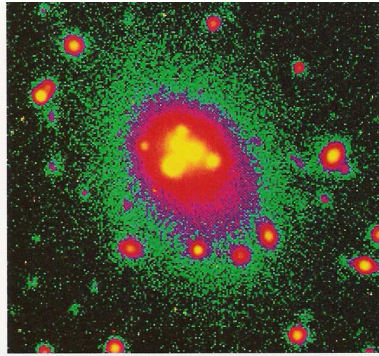
FIGURE 17.26 The central galaxy of the cluster Abell 3827, shown here in false color, has multiple clumps of stars that probably once were the centers of individual galaxies.
