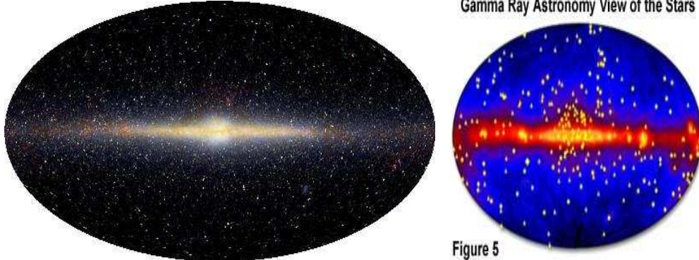
Gamma Ray Astronomy View of the Stars
